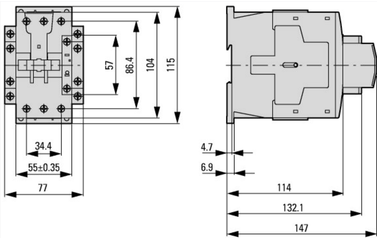
Contactor with auxiliary contact module
